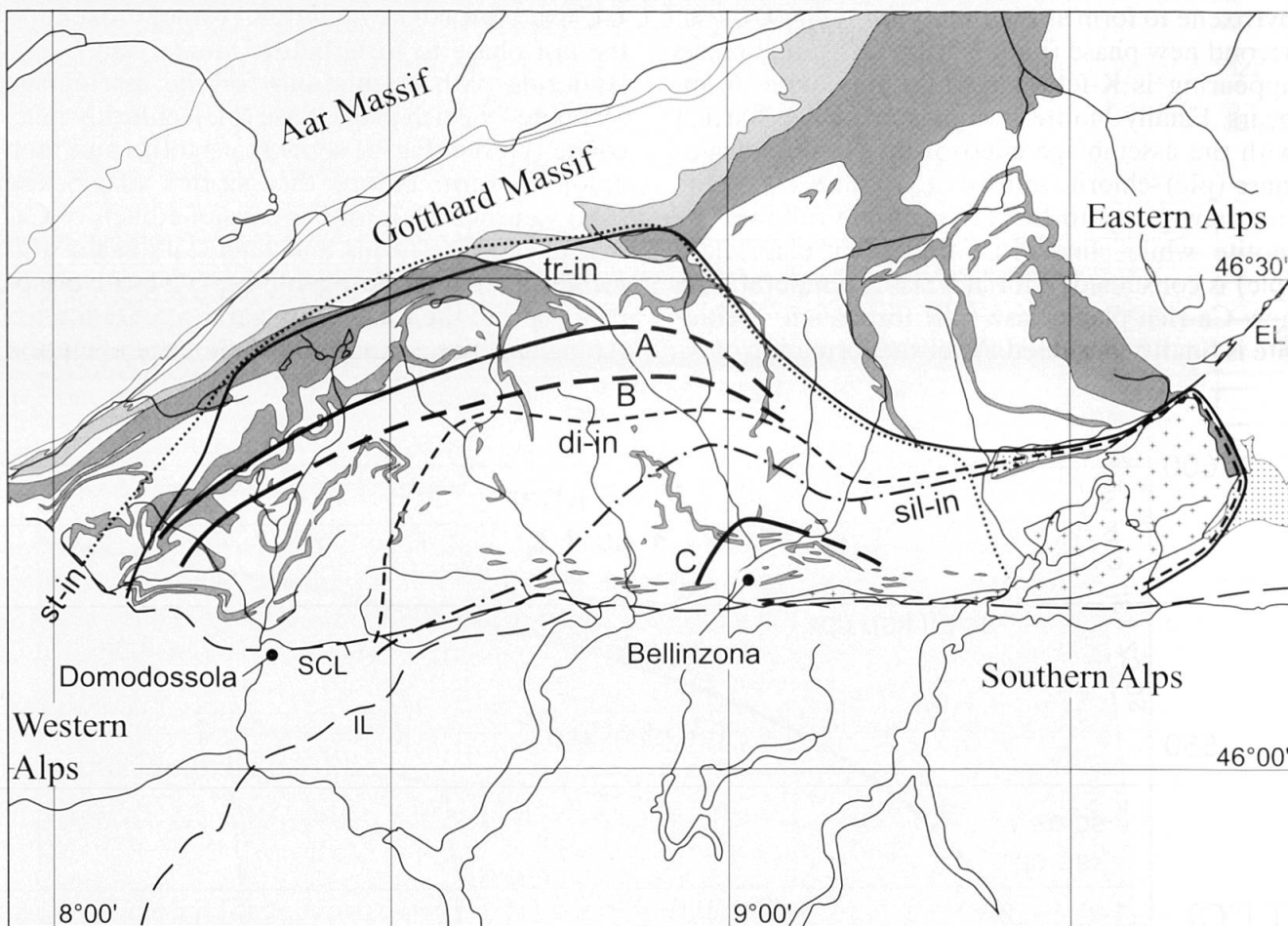
Fig. 10 Schematic map of the Central Alps from Fig. 1 showing the approximate geographic location of the transition clinzoisite+plagioclase to scapolite-bearing assemblages (A), the appearance of K-feldspar (B) and the appearance of clinopyroxene (C) in calc-schists, superimposed on the Geological map of Switzerland (1980).
