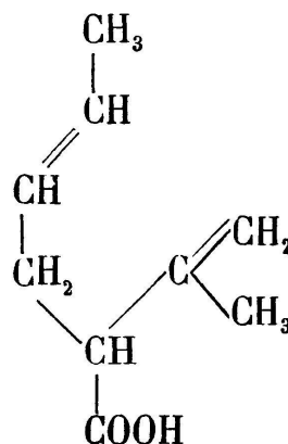
Acide C_9H_{14}O_2
