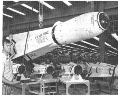
AGM-65 Maverick
