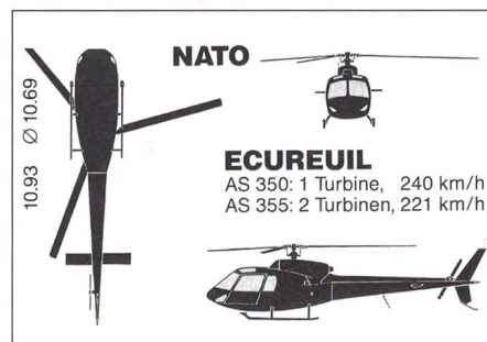
Ecureuil
