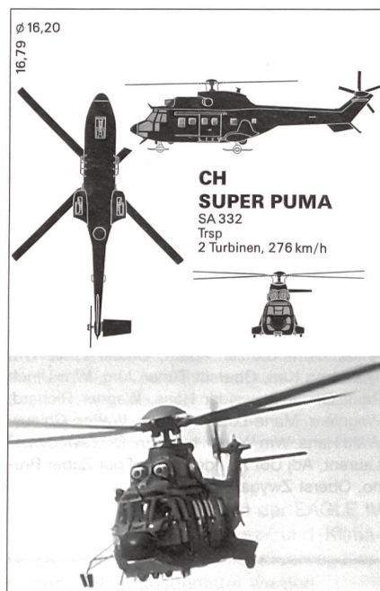
SUPER PUMA
