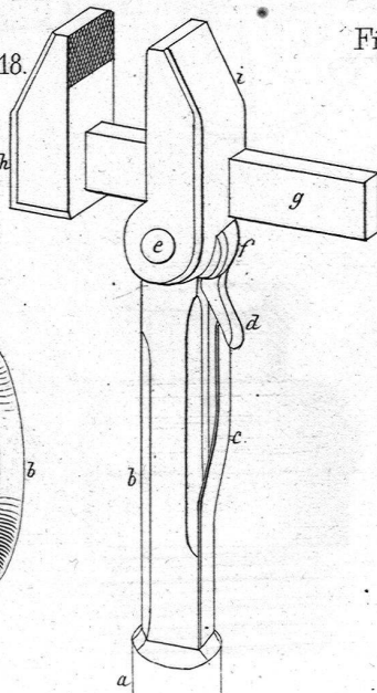
Whiterell's Schraubenschlüssel.
