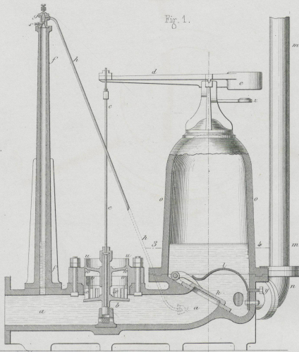
Bolée's Stosshöher.
