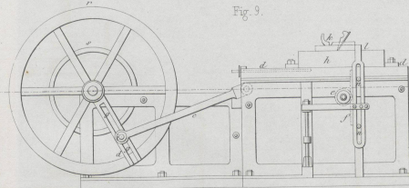
Wisna's Zundholzbohrmaschine.
