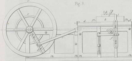
Wisna's Zundholz Hobelmaschine.
