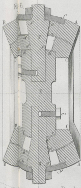
Reveley's Dampfhammer.
