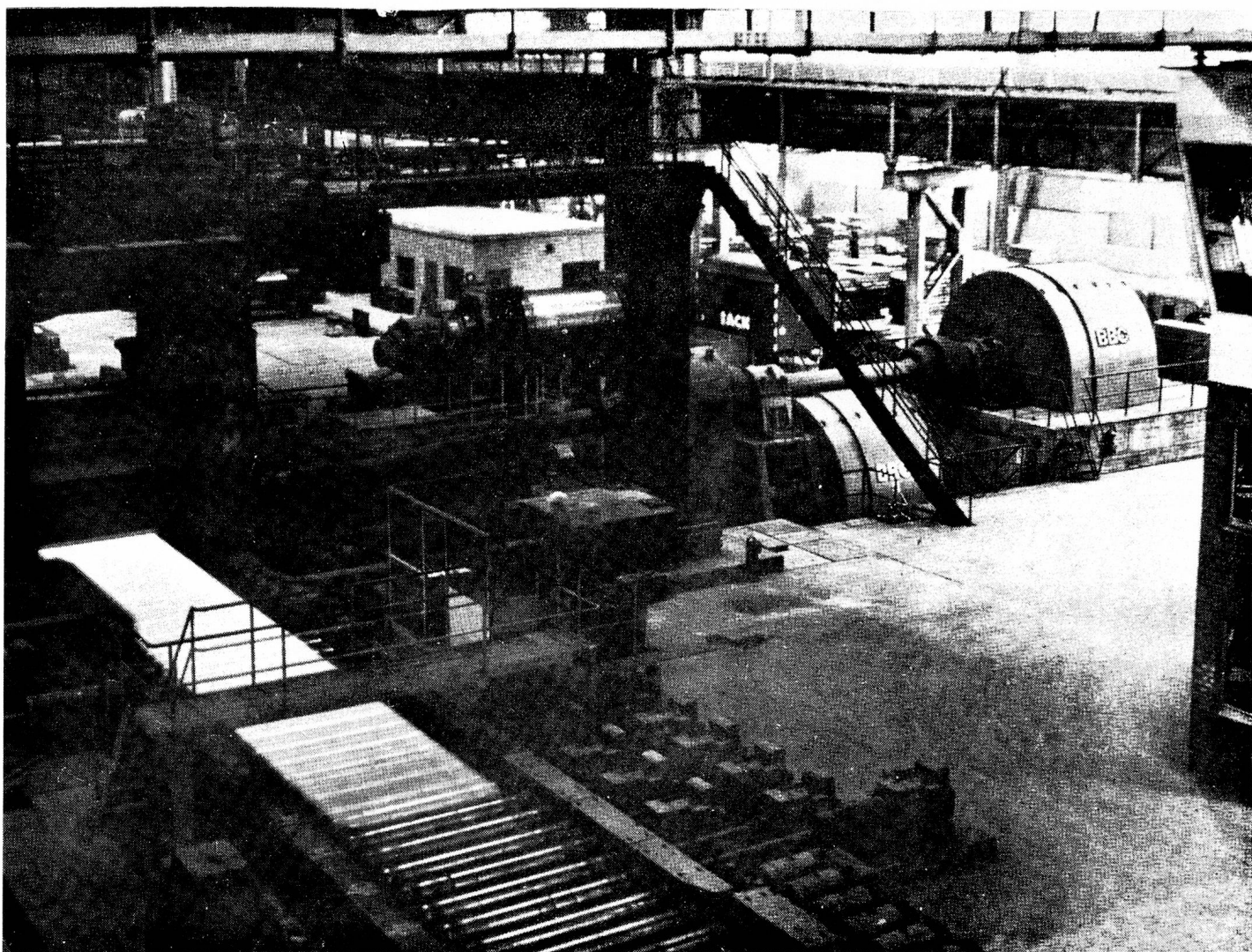
Two BROWN BOVERI 4600/11,400 H.P., 55/130 r.p.m. reversing drives installed in a steel mill.
