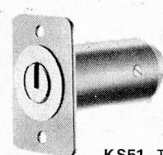
KS51. Two-pole 4 amps at 250 VAC.
