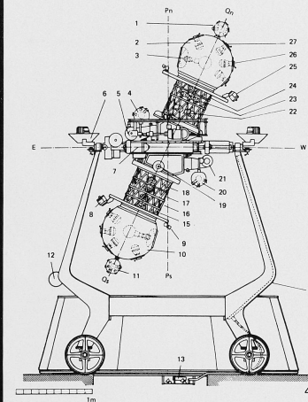
Drawing of the Zeiss planetarium projector unit in the Swiss Museum of Transport, Lucerne
