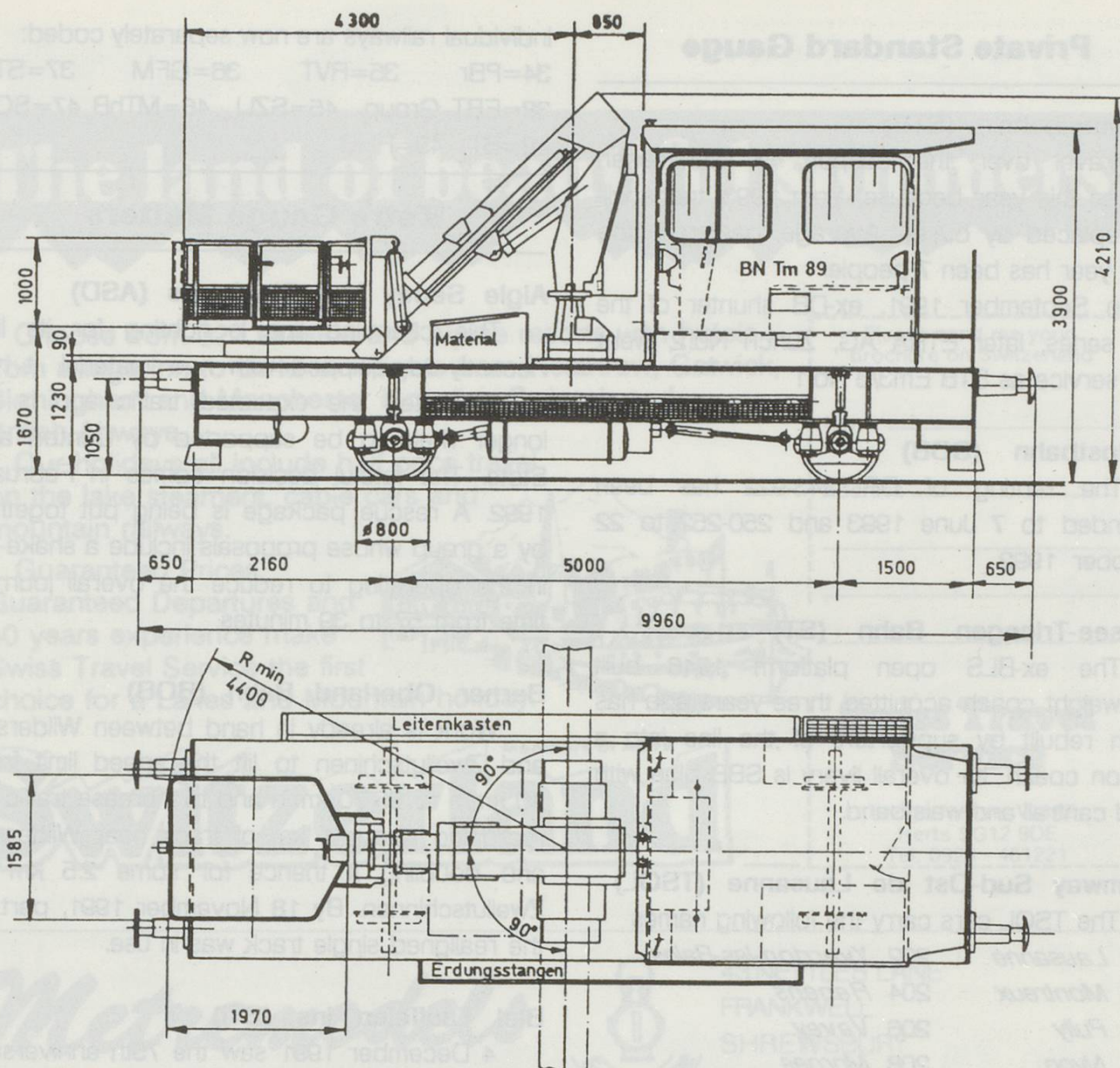
BLS Tm2/2 tractor Hugo
