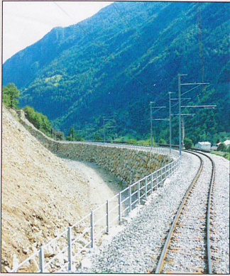
Following the problems at Brusio early in 2009, this view shows some of the repairs to the track. PHOTO: Peter Dixon.
