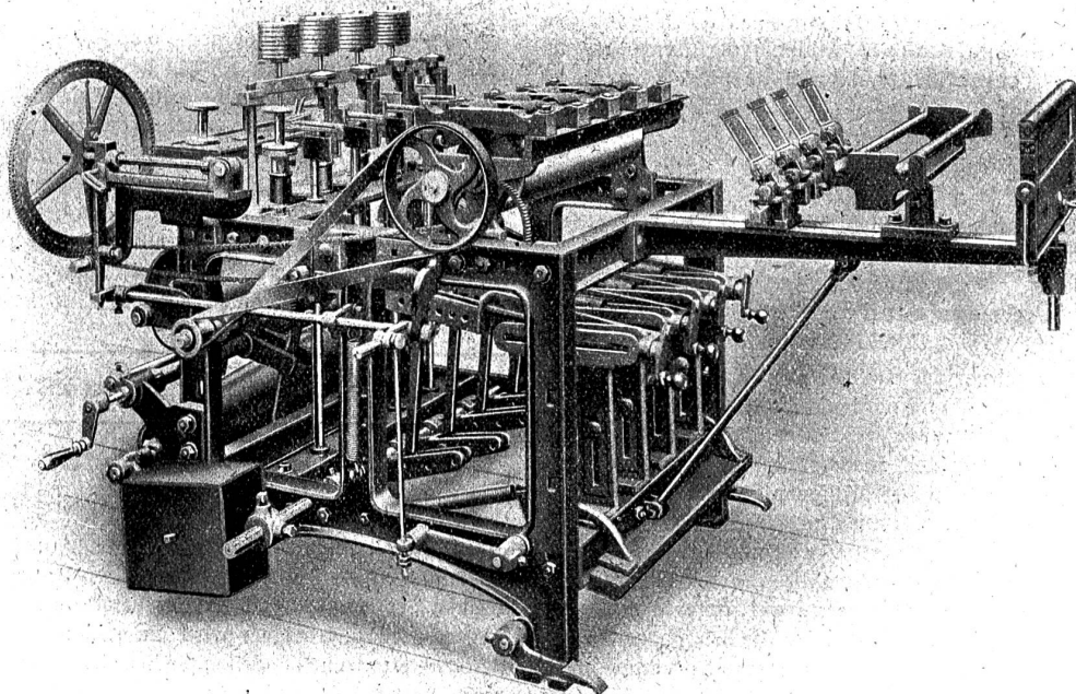
6. Bandzettelmachine.
