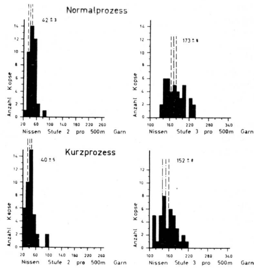
Abb. 12 Nissen IPI
