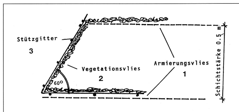
1 = Armierungsvlies 2 = Vegetationsvlies
