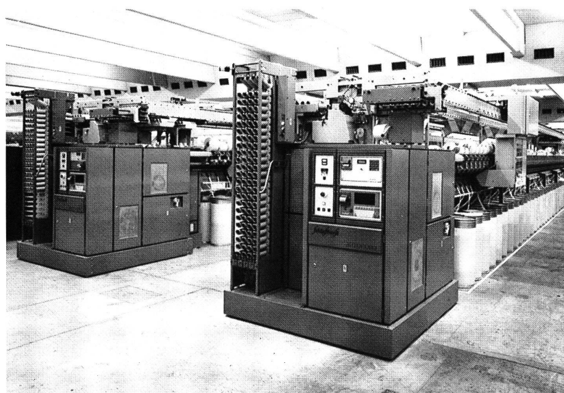
Rotor-Spinnspul-Automat Autocoro 288
