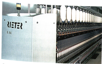
ComforSpin-Maschine K 44
