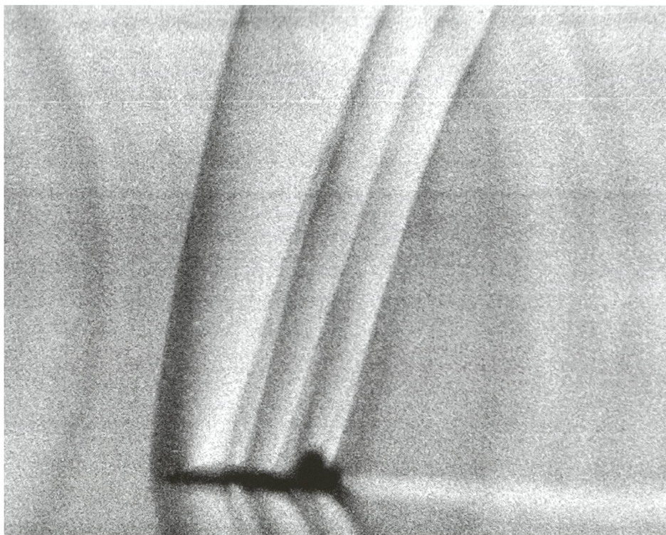
Schlieren photograph of T-38 shock waves at Mach 1.1, 13,000 feet [photo: Dr. Leonard Weinstein, 1993]
