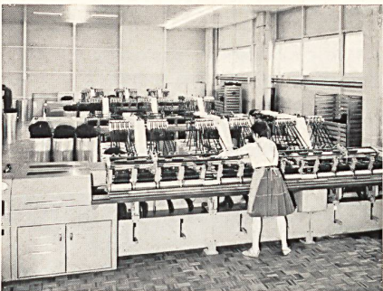
Ultra-modern frame for fine drawing in a worsted mill
