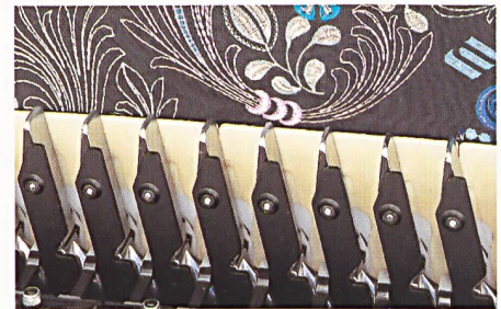
Pentacut thread cutting device on the shuttle side.
