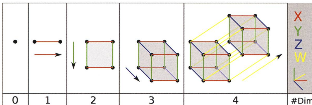
Hypercube construction: First four dimensions (from http://wikipedia.org/wiki/Hypercube )
