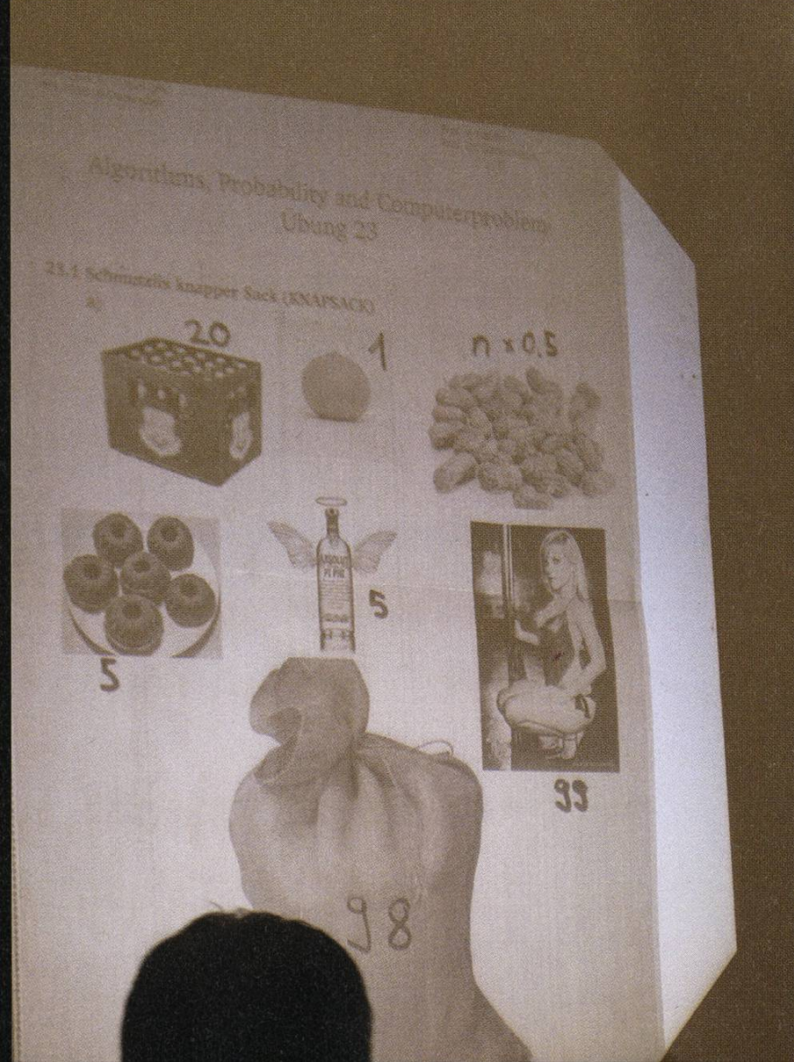
5. Semester: Algorithms, Probability and Computing Ueli Maurer
