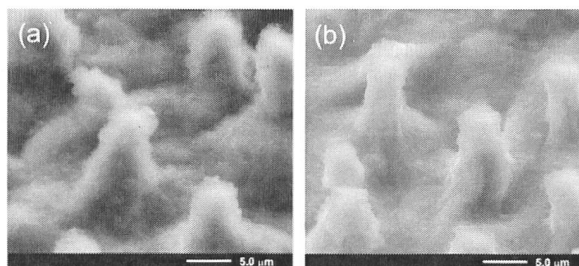
Figure 1. An exact replica (b) of a natural lotus leaf (a). A fresh leaf has been coated with the silicon-based polymer poly(dimethylsiloxane), creating a negative imprint. A second layer of the polymer again created the positive replica showing the same characteristics as the natural leaf surface. Reprinted with permission from Langmuir 2005, 21, 8978–8981. Copyright 2005 American Chemical Society.
