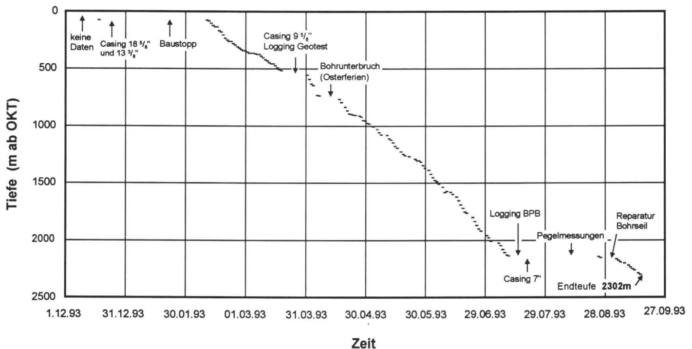
Fig. 1: Bohrfortschritt
