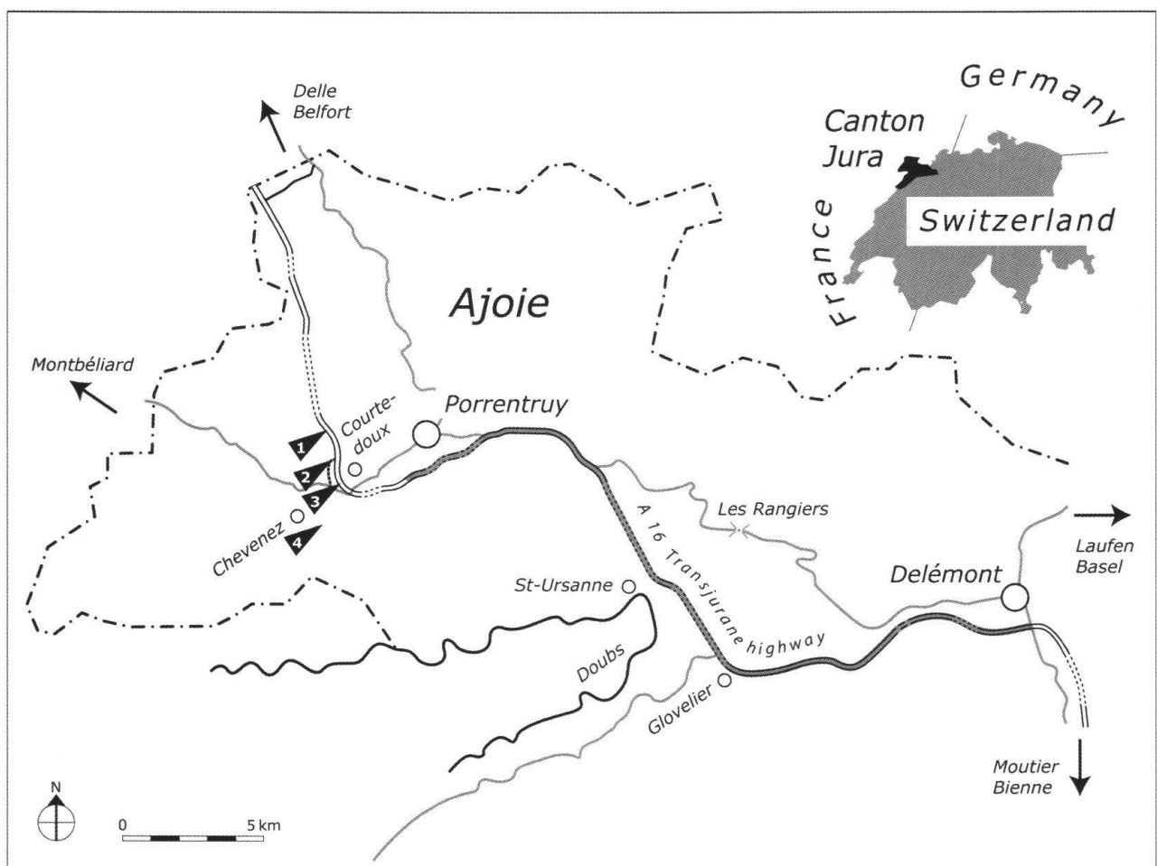
Fig. 4: Location of the tracksites along the future Transjurane highway. From north to south 1: Courtedoux - Béchat Bovais and Courtedoux - Bois de Sylleux, 2: Courtedoux - Tchâfoué and Chevenez - Combe Ronde, 3: Courtedoux - Sur Combe Ronde and Chevenez - Crât, 4: La Combe quarry (Chevenez).
