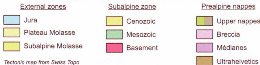
Tectonic map from Swiss Topo
