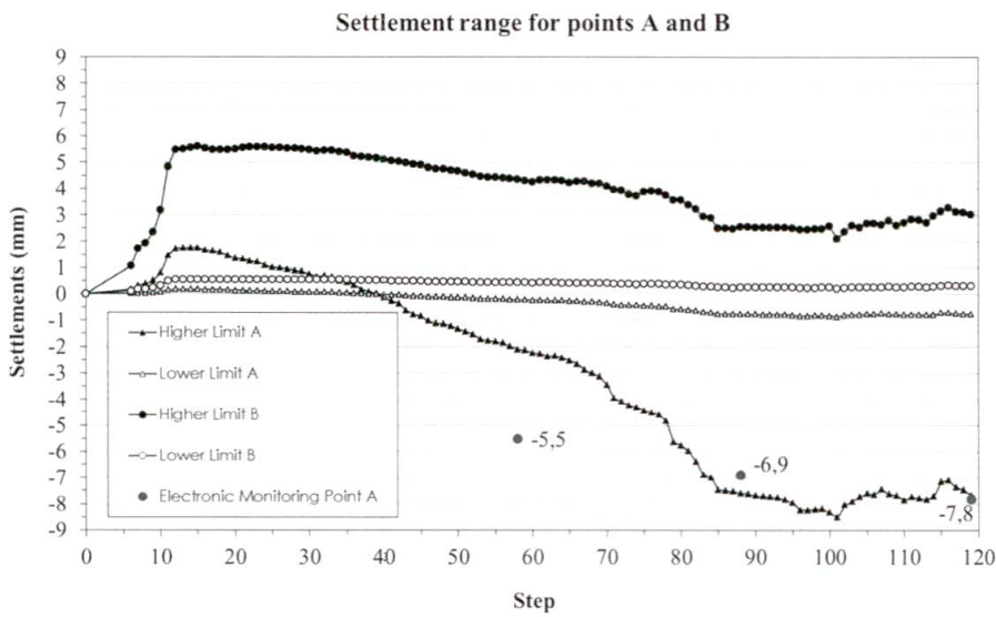
Fig. 6: Time-settlement calculated curves and real measurements at Città di Castello tower.
