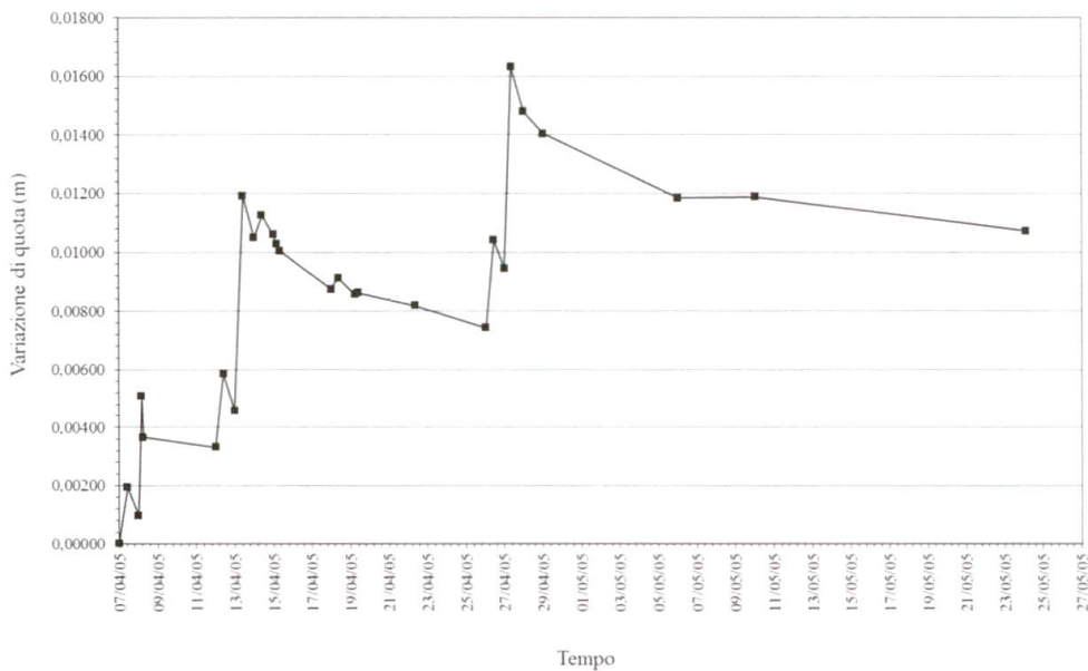
Fig. 9: Time-displacement measured curve for «point 17» [x-axis: date, y-axis: displacement rates in m].
