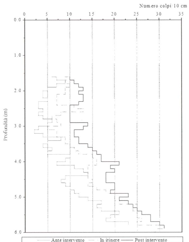
Fig. 4: Penetrometer tests before (light grey) and after (dark grey) intervention at Palatium Vetus [x-axis: number of strokes per 10 cm, y-axis: depth [m]].
