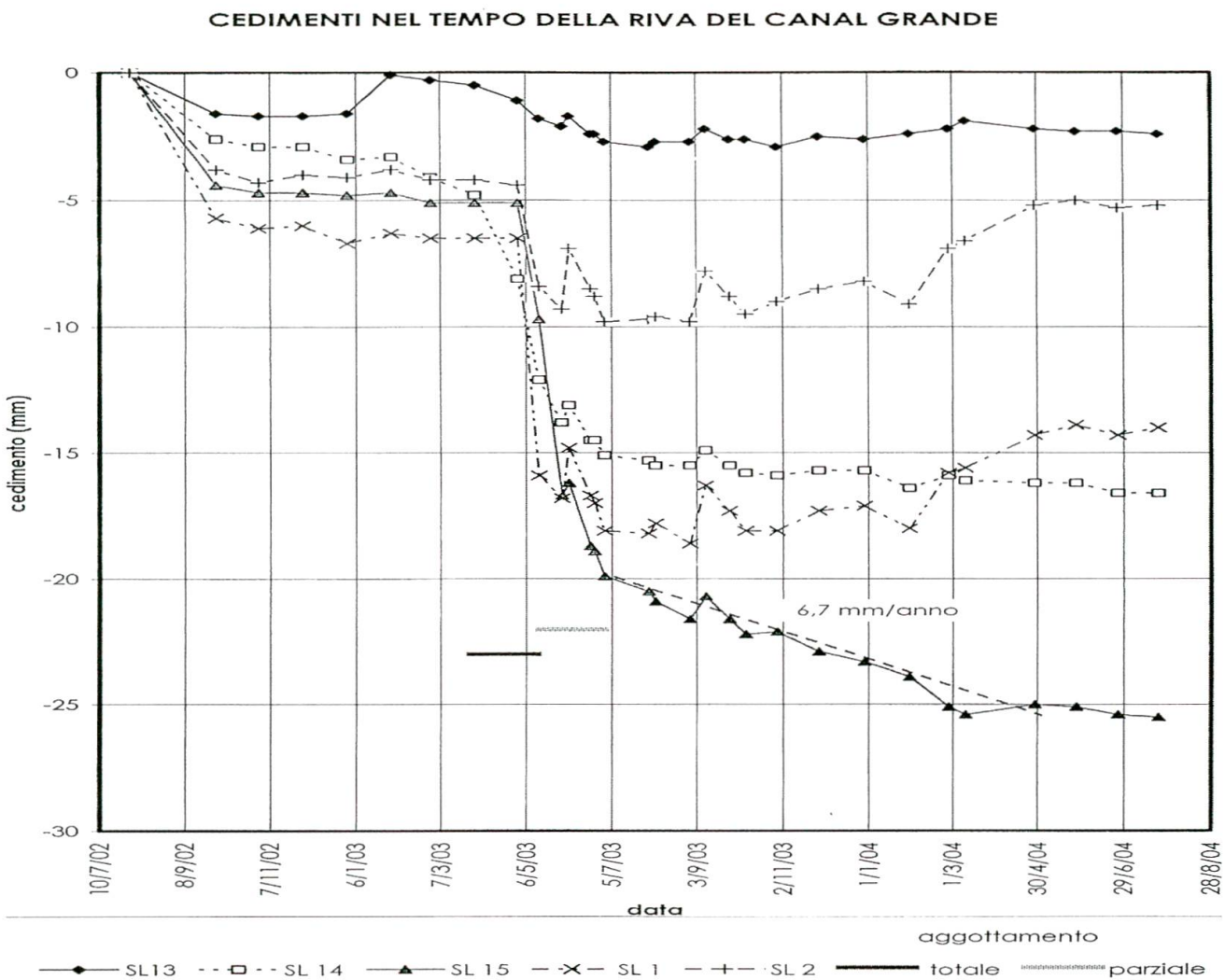
Fig. 8: Time-settlement curves of several anchorages (x-axis: date, y-axis: settlement in mm).
