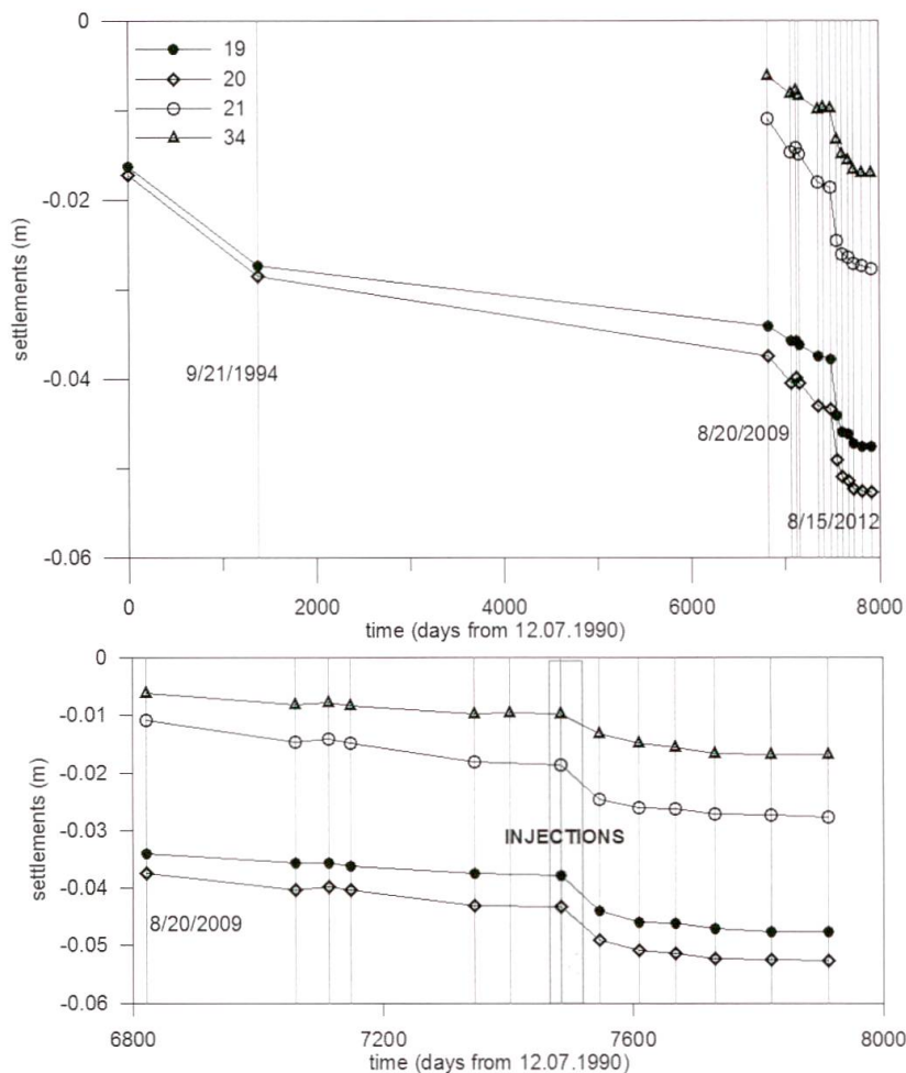
Fig. 14: Above: time-settlement curves of several anchorages. Below: enlargement of the measurements just before and after intervention.
