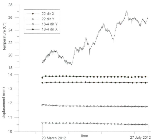
Fig. 16: Time- displacement-temperature curves for two cracks (in X and Y directions).
