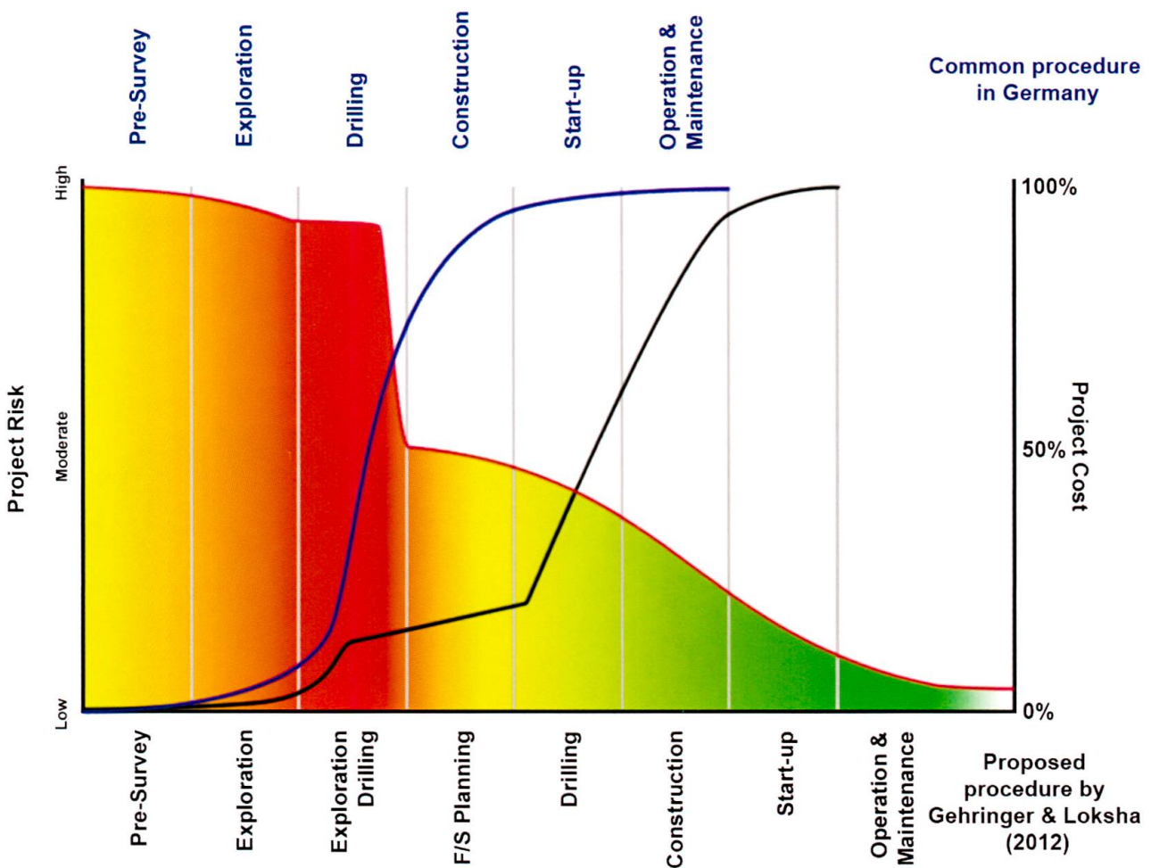
Fig. 3: Comparison of the cost development and project phases of deep geothermal projects as proposed by Gehring & Loksha (2012) in black font and black curve and the cost development and project phases reflecting the actual common procedure of deep geothermal projects in Germany in blue font and as blue curve in correlation to the development of the project risk. The further the project proceeds the higher the bankability becomes.
