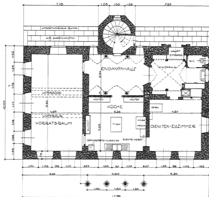
Grundriß Erdgeschoß
