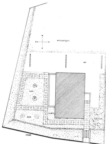
Situationsplan 1:500
