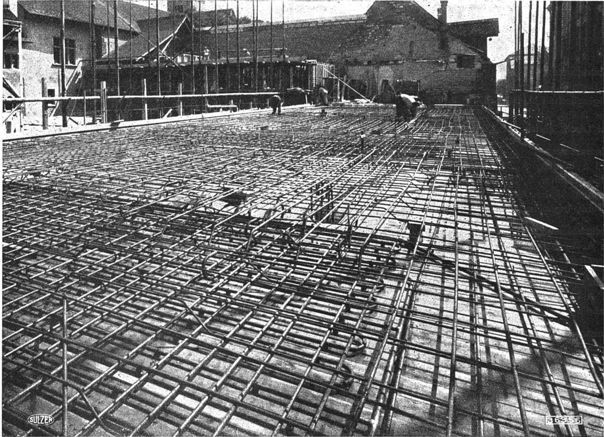
Strahlungsheizung, System Crittall, in Montage. - Museum zu Allerheiligen, Schaffhausen
