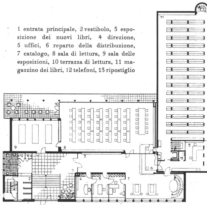
Piano terreno 1:400
