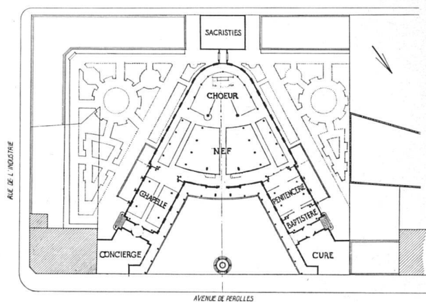
Situationsplan 1:1500
