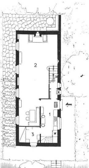
Erdgeschoß 1:300 / Rez- de-chaussée / Ground floor
