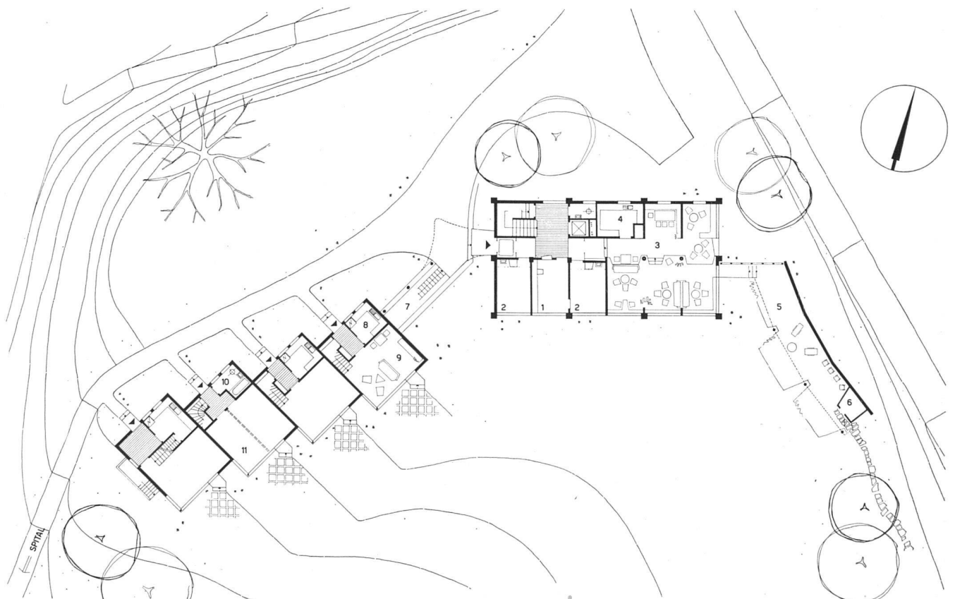
Erdgeschosse 1:500 | Rez-de-chaussée | Ground floor plans
