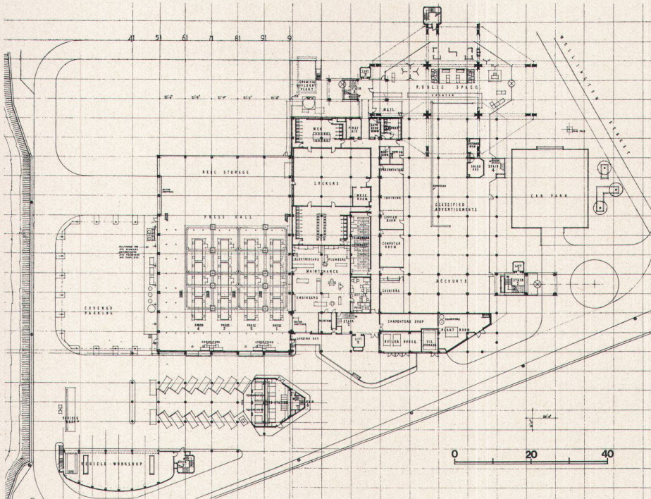
Grundriß Erdgeschoß
