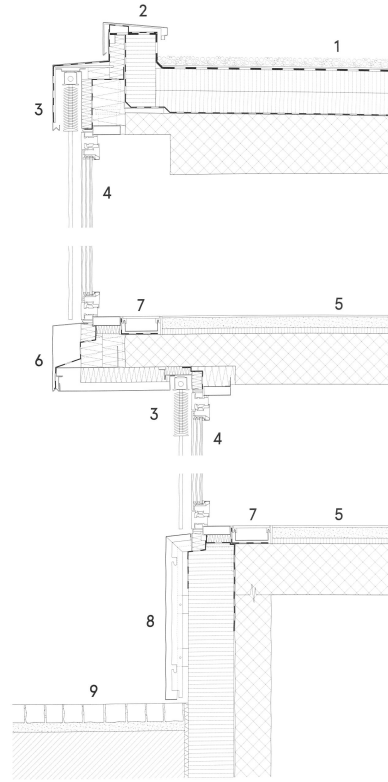
Coupe constructive
