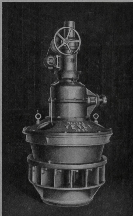
Kaplan-Turbine
