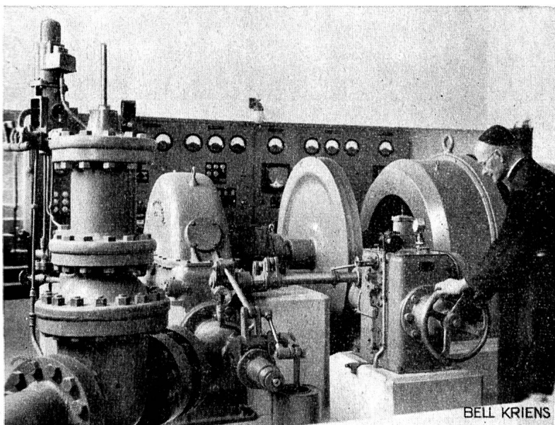
600 PS Peltonturbine
