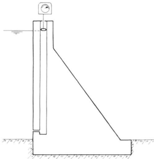
Reference number 1.000-2. Float to measure the reservoir water level.
