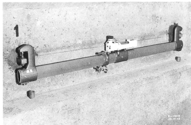
Reference number 2.150(1). Clinometer placed on the two reference points.
