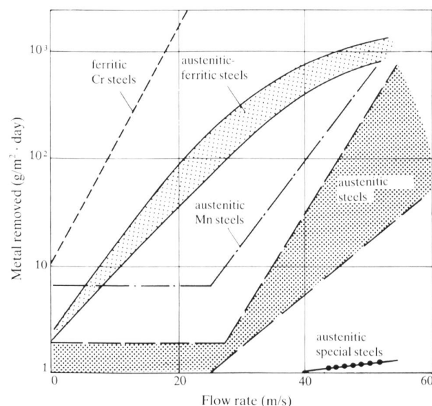
Fig. 8.12 (p. 266). Rates of corrosion of stainless steels as a function of flow rate in m/s. Medium: injection water, 60°C, 270000 mg/l dissolved salts, pH 4.5.
