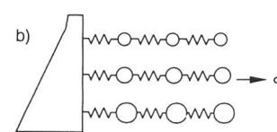
Halbunendliches Feder-Masse-System
