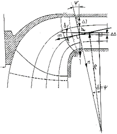
Fig. 1. Guide vane outlet-flow towards the runner inlet for calculation of the blade-inlet angles for the different stream surfaces. (Note: n-direction is normal to the meridian flow direction with positive value towards the centre of the curvature radius \rho .)
