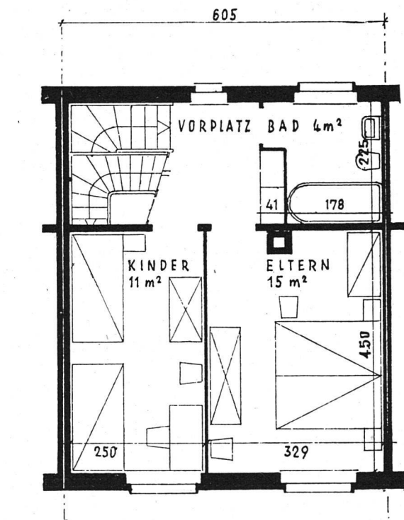
Grundriß: 1. Stock
