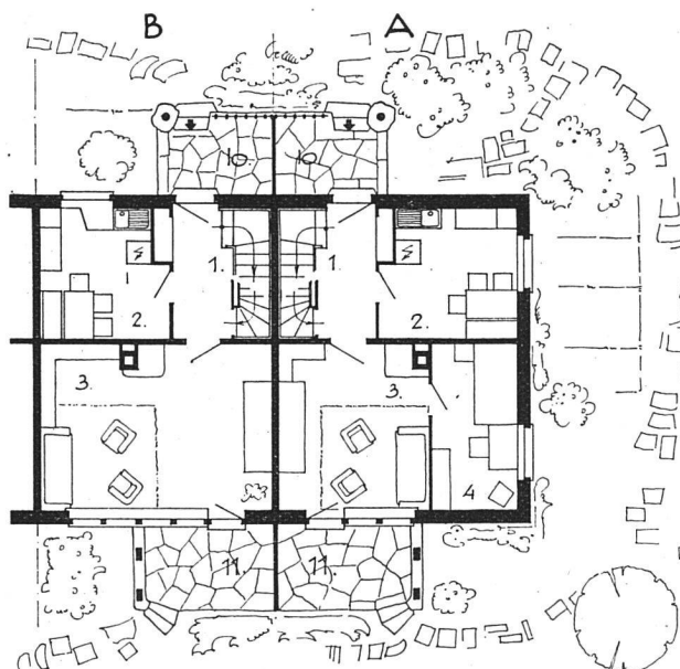
Grundriß Erdgeschoß
