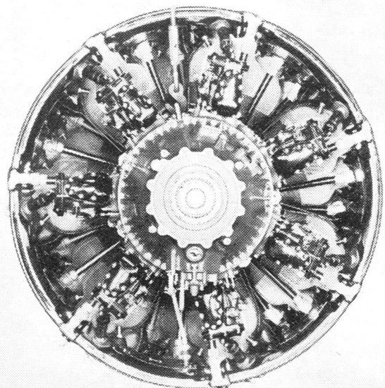
28-Zyl.-Pratt & Whitney-Sternmotor.
