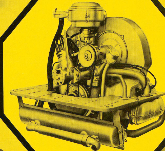
Notstrom-Aggregat
